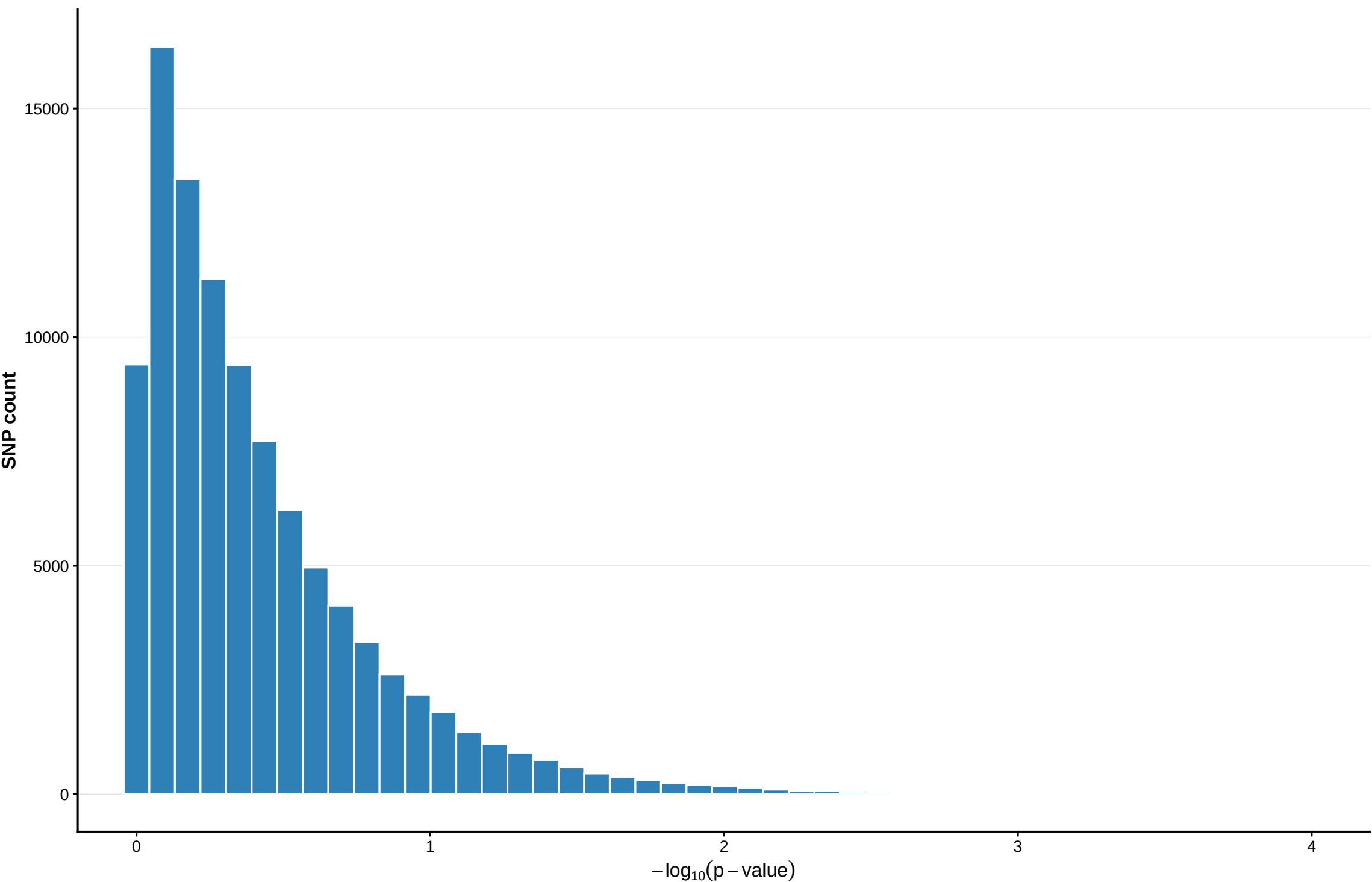
Distribution of -\log_{10}(\text{p-values})
